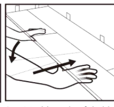
Step 4: Lock long edge of plank by inserting tongue into groove at an approximate 15 degree angle and drop into place. Next slide toward end of previously installed plank until the tongue touches the groove.
